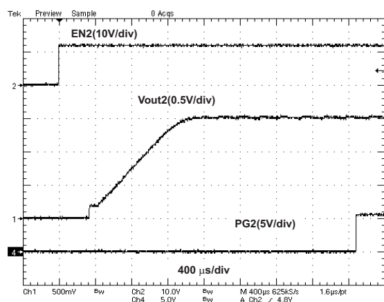
Figure 11. VO2=1.5V, PG2
