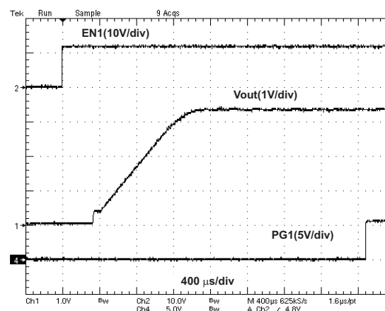
Figure 10. VO1=3.3V, PG1
